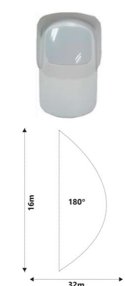
Outdoor KNX Microwave Sensor
