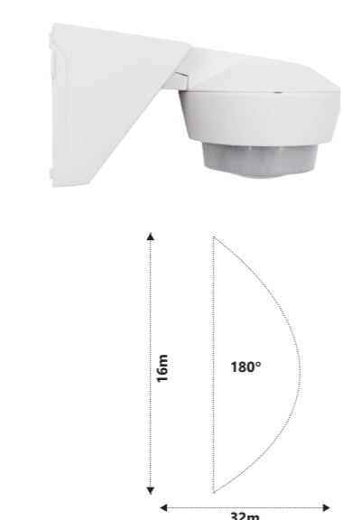
Outdoor KNX Movable Motion Sensor
